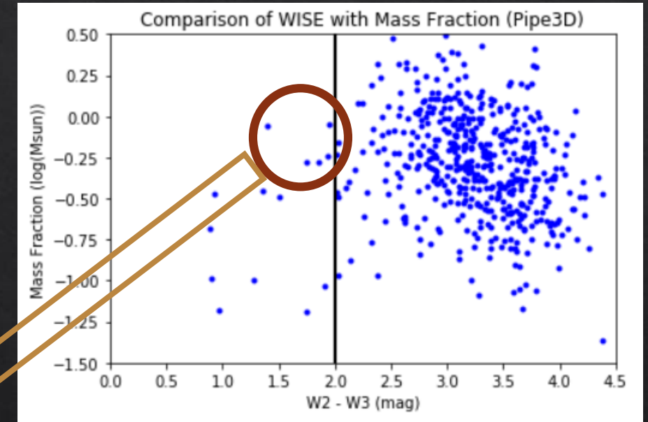
Fig: HI Mass Fraction vs W2-W3
