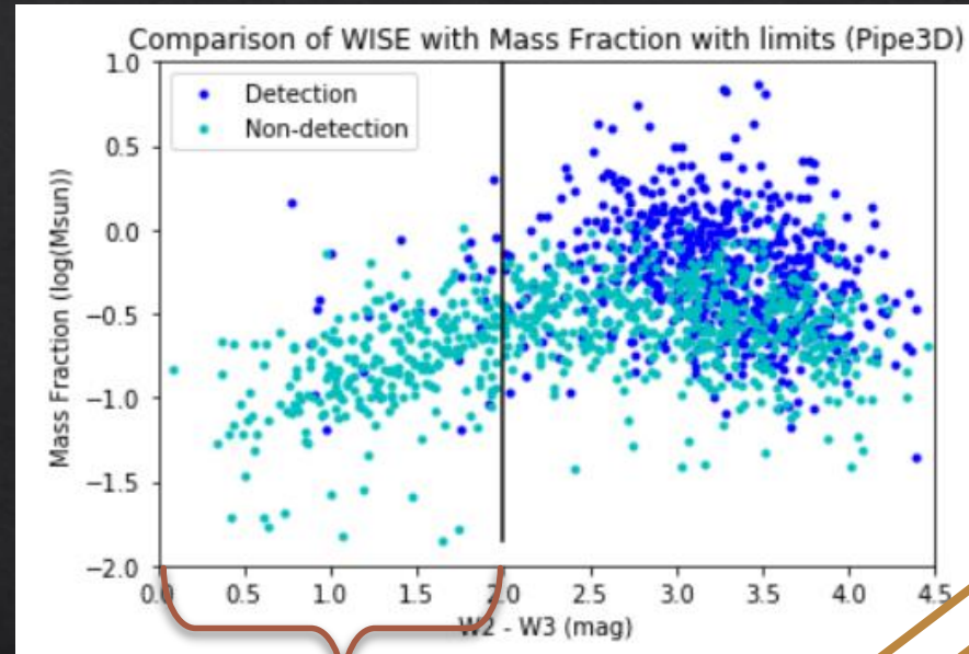
Low SFR Region (Brown et al. 2017)
